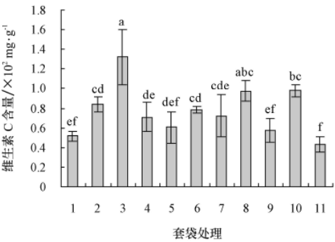
图 3 不同套袋处理对采后香蕉维生素 C 含量的影响 Fig.3 Effects of different bagging treatments on vitamin C levels of harvested banana fruits
