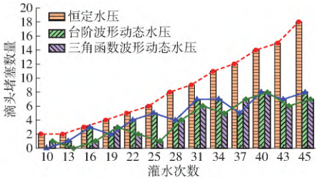
图 4 不同水压模式下滴头堵塞数量与灌水次数的关系 Fig. 4 Relationship between number of clogged emitters and irrigation time with different pressure patterns
